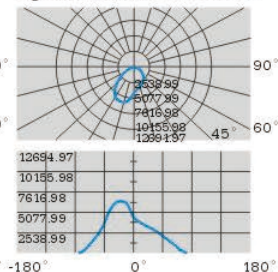
Light Distribution Curve C90/C270
