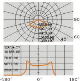
Light Distribution Curve C0/C180
